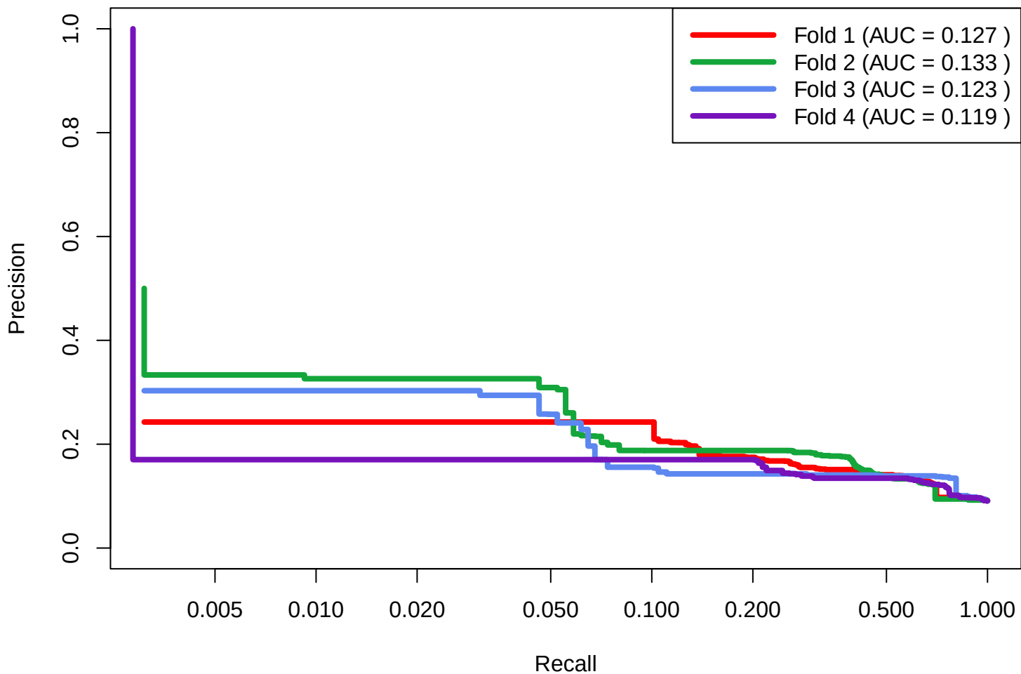
SPELL Network 50 Dataset: 50x20x1 Validation
